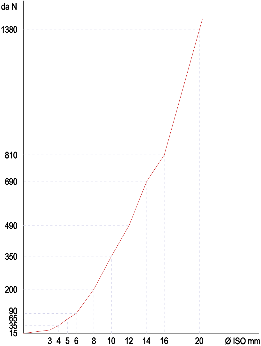
*Tensile strength at break (Nylon 66)
